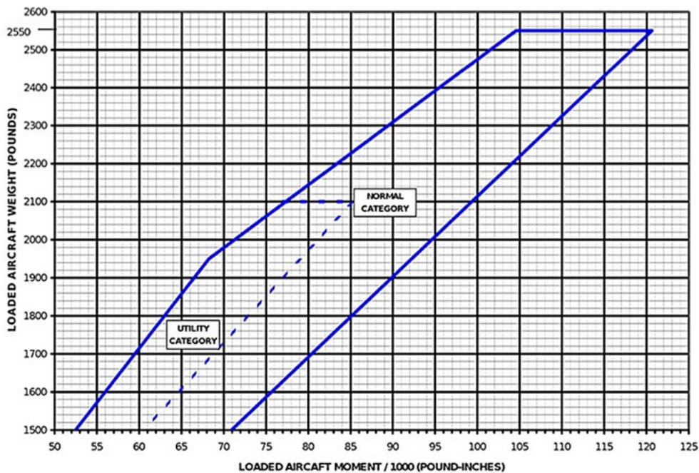
CENTER OF GRAVITY MOMENT ENVELOPE
